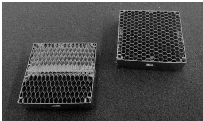
MAJR Shield© US Patent No.:7,589,968 EMI/RFI Shielding and Thermal Management
