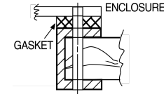
Figure 5 Recess Mount Style 3036
