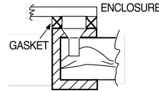
Figure 6 Through Hole Style 3033
