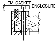
Figure 6 Through Hole Style 3033
