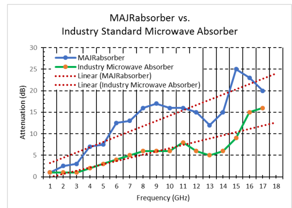
Figure #3 Attenuation (dB) vs. frequency (GHz)
